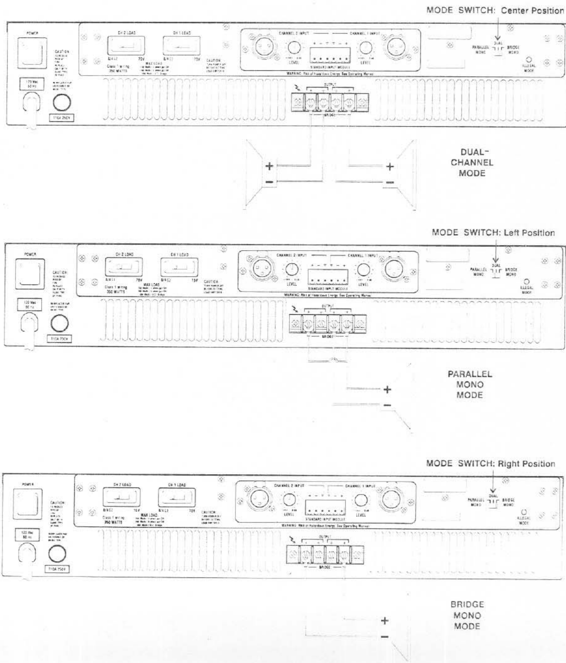
Figure 2—Output Configurations
